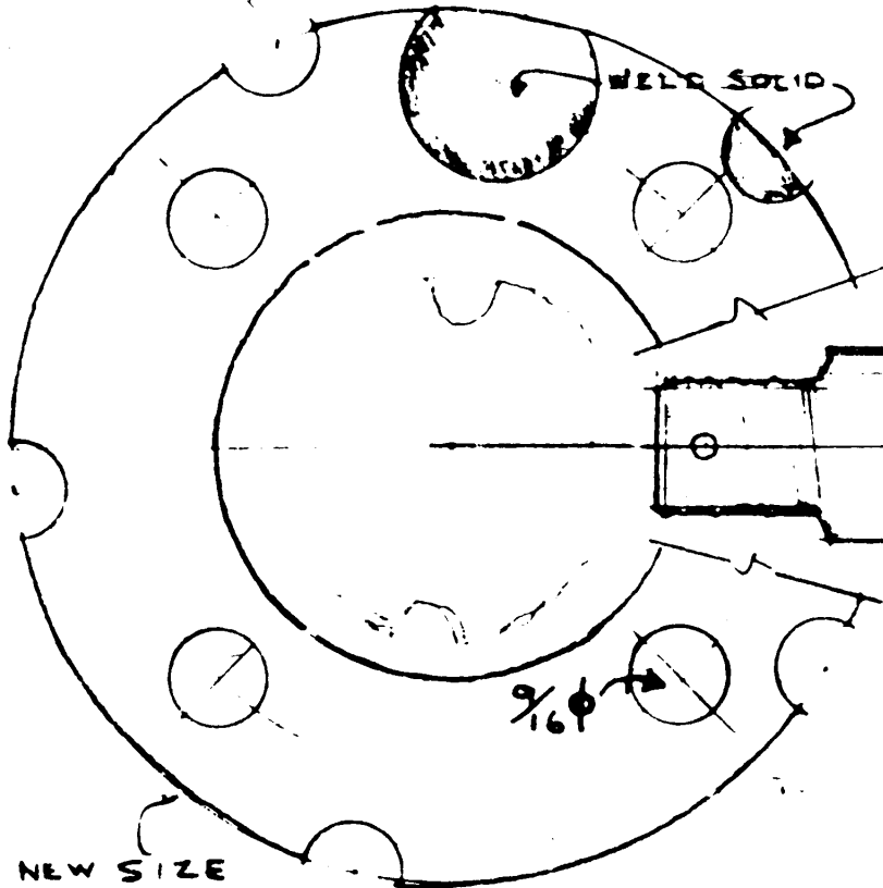
FACE OF FLANGE SHOWING BOLT CIRCLE
